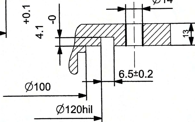
DETAIL-X
