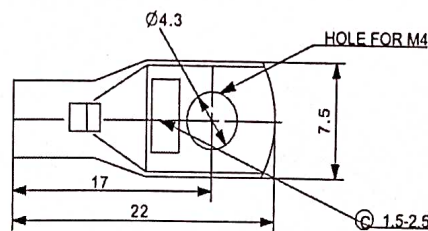
CABLE LUG SIZE 1.5-2.5/M4 ID NO. 3EHP470026P0014 FIG. NO. 26
