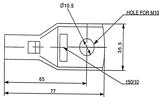
CABLE LUG SIZE 150/M10 ID NO. 3EHP470026P3710 FIG. NO. 25
