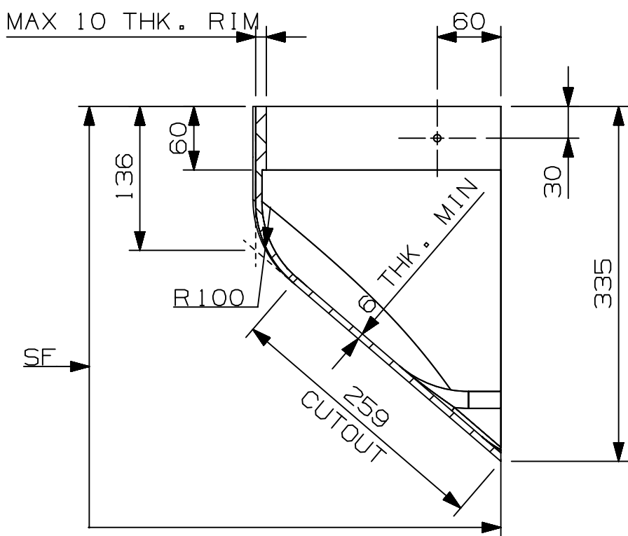
SECTION C-C SCALE 1:5
