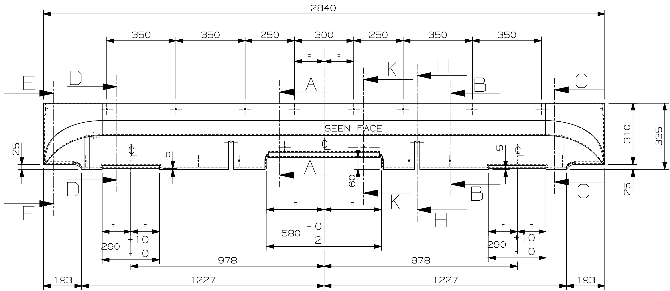
PLAN VIEW
