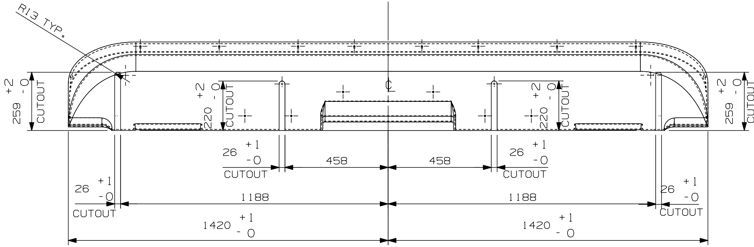
VIEW G
