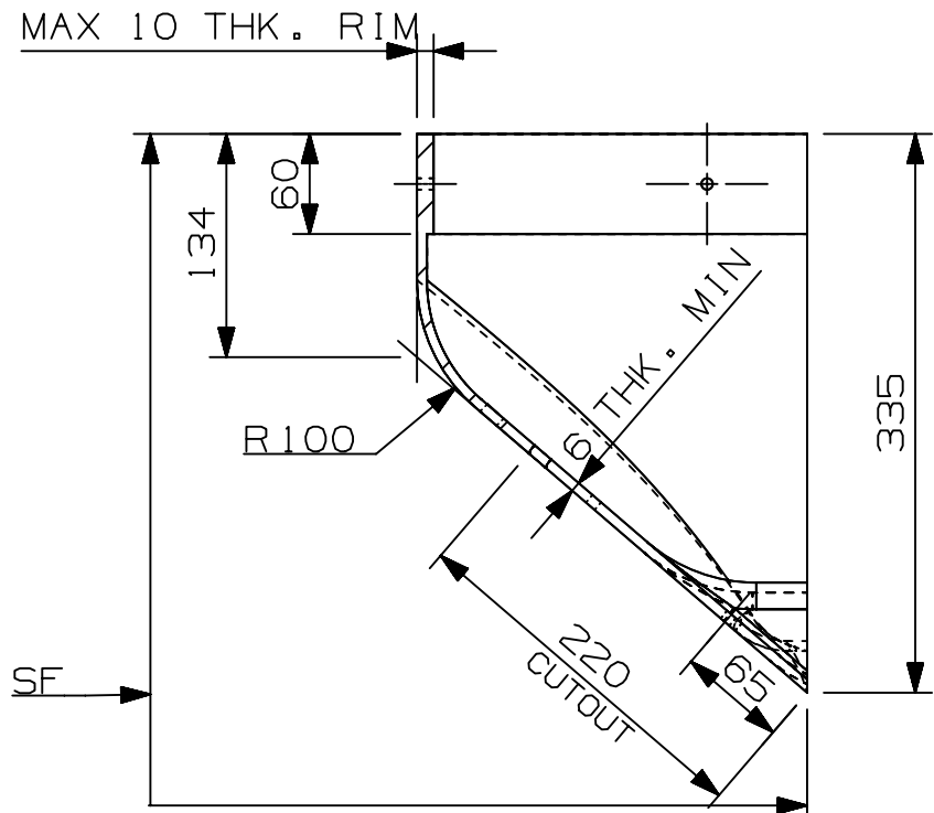
SECTION H-H SCALE 1:5
