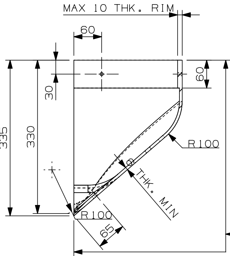
SECTION D-D SCALE 1:5
