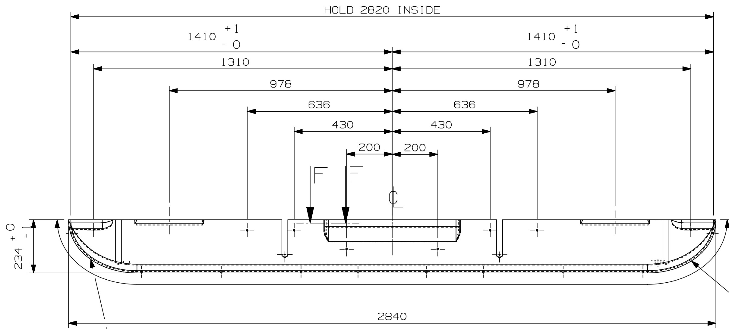
PLAN VIEW
