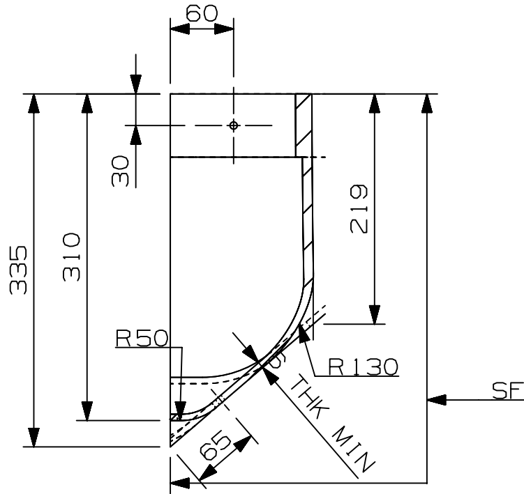
SECTION B-B SCALE 1:5
