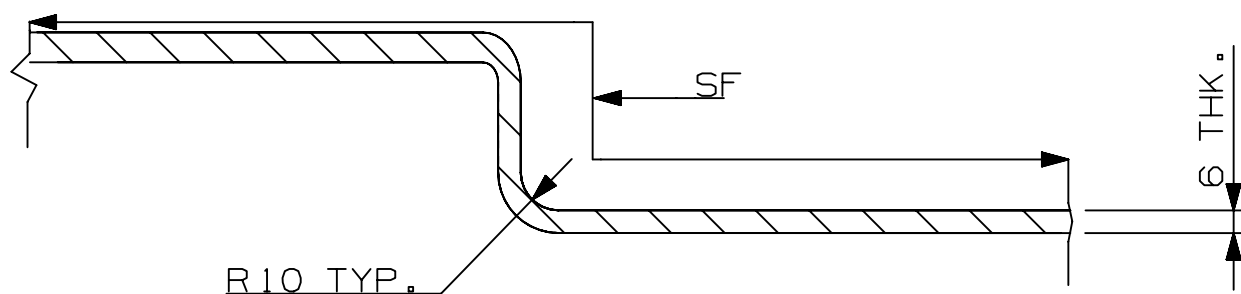
SECTION F-F SCALE 1:2
